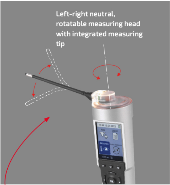
Long, stepped, flexible, deflectable measuring tip made of flexible, tissue-friendly material
